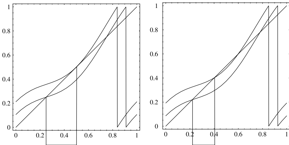
Figure 1. The random diffeomorphisms f_\alpha given by (2); drawn are the extremal graphs f_\alpha(\cdot, \pm 1) for \alpha = \alpha_0 and slightly below (see text). The intervals indicate the support of the stationary measure.
